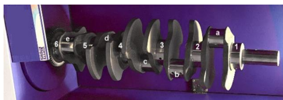
Fig. 1. 1, 2, 3, 4, 5, 6 – fusuri paliere, a, b, c, d, e – fusuri manetoane
